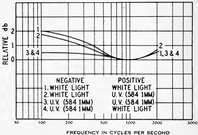
FIG. 9. Low-end frequency characteristics for various recording and printing conditions.
